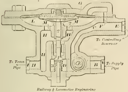
Fig. 1.—VALVE FOR TRIPLE VALVE TESTING DEVICE.
